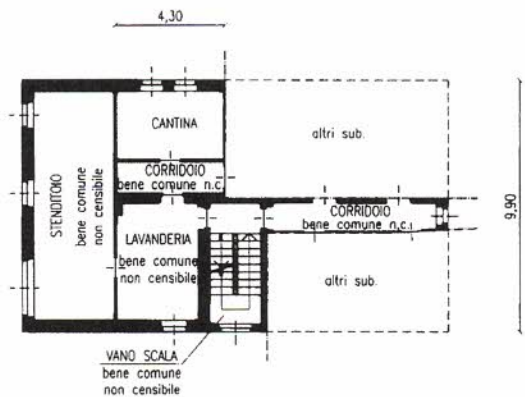
PIANO SEMINTERRATO h. 2,80
